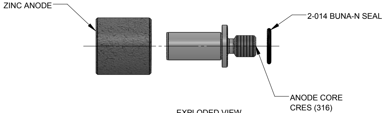
EXPLODED VIEW
